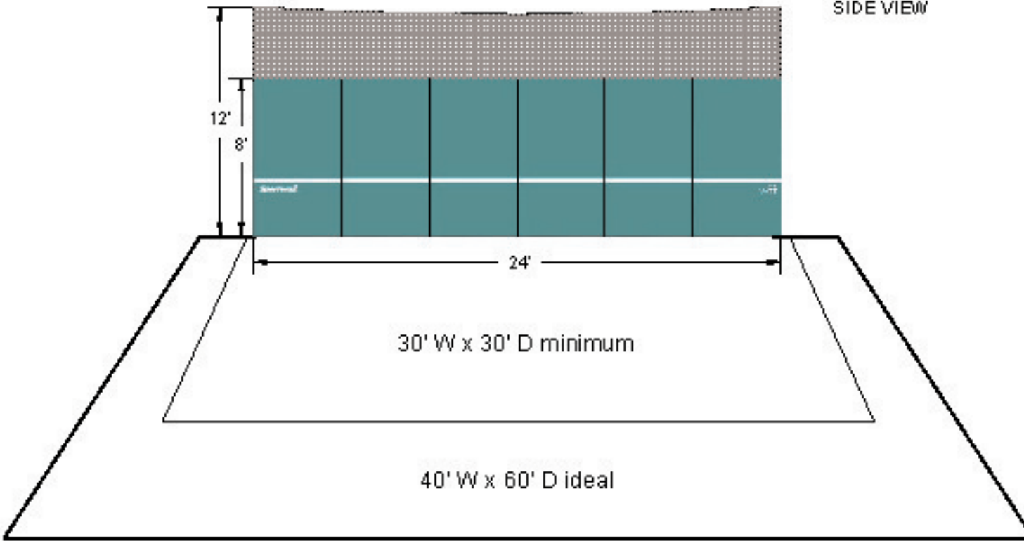
SIDE VIEW
